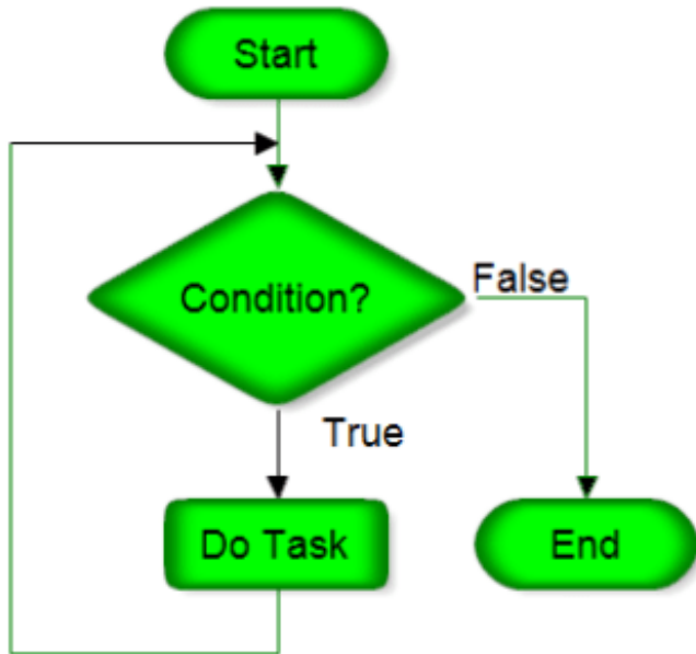
While Loop
